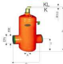
Welded/Flange Technical Details Of Connection.
